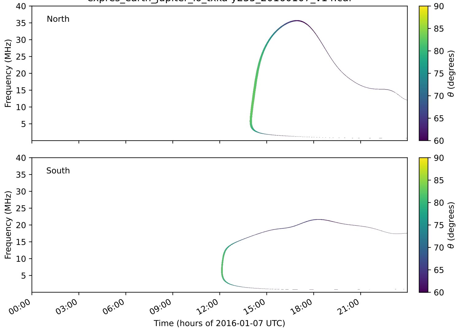
expres_earth_jupiter_io_txka-y235_20160107_v14.cdf
