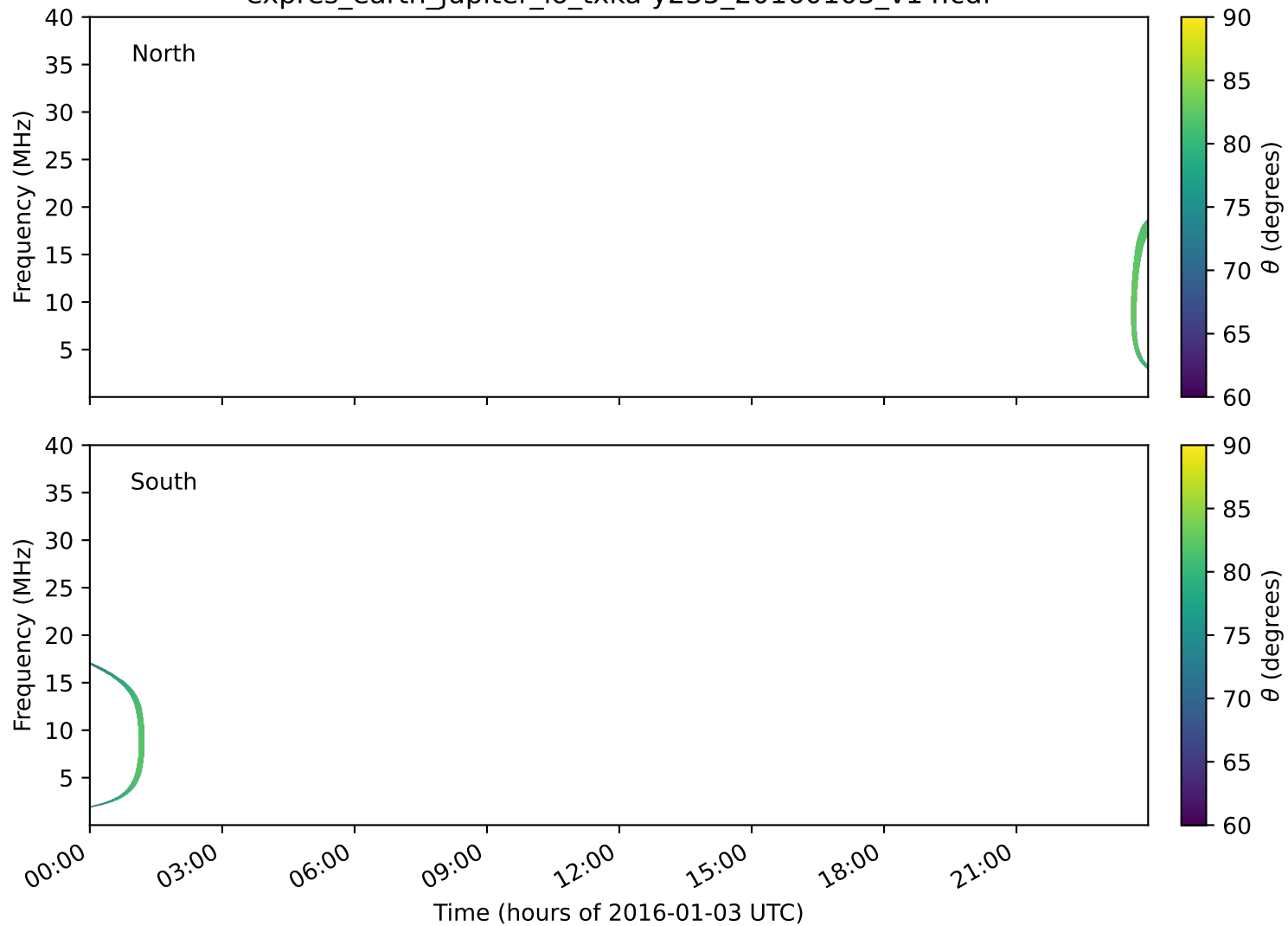
expres_earth_jupiter_io_txka-y235_20160103_v14.cdf
