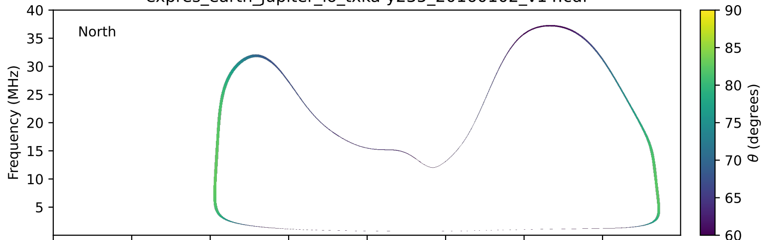
expres_earth_jupiter_io_txka-y235_20160102_v14.cdf
