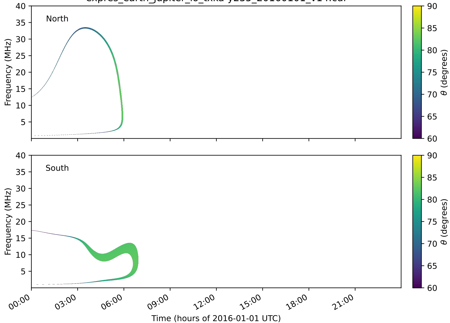
expres_earth_jupiter_io_txka-y235_20160101_v14.cdf
