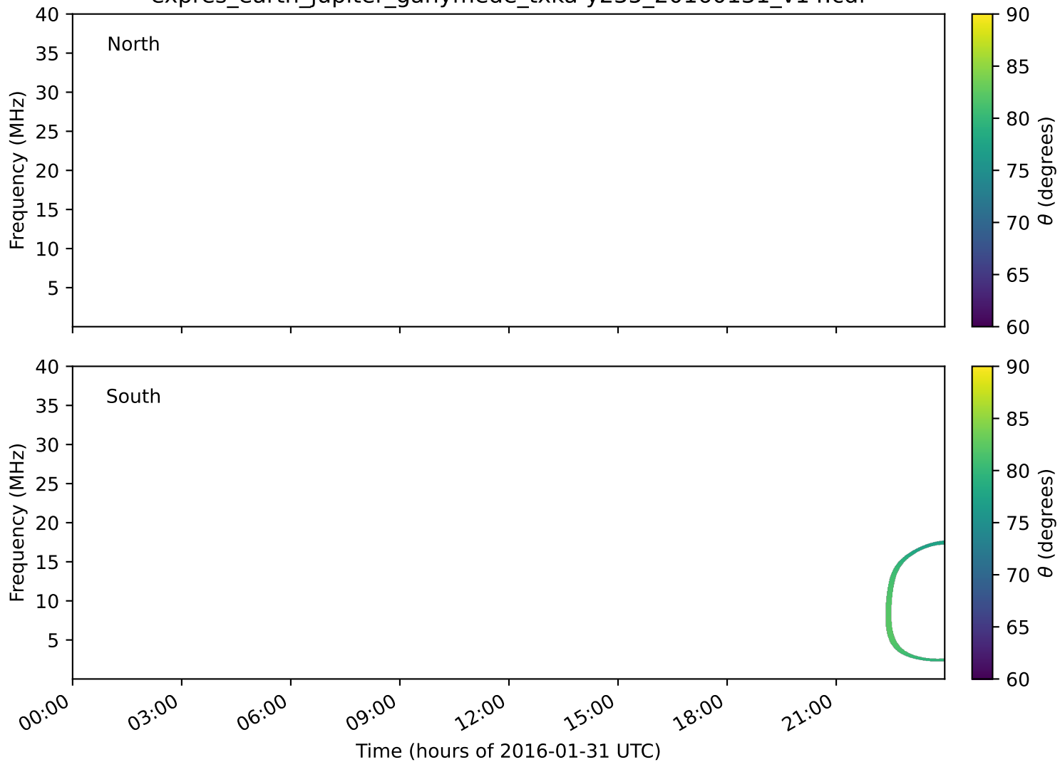
expres_earth_jupiter_ganymede_txka-y235_20160131_v14.cdf
