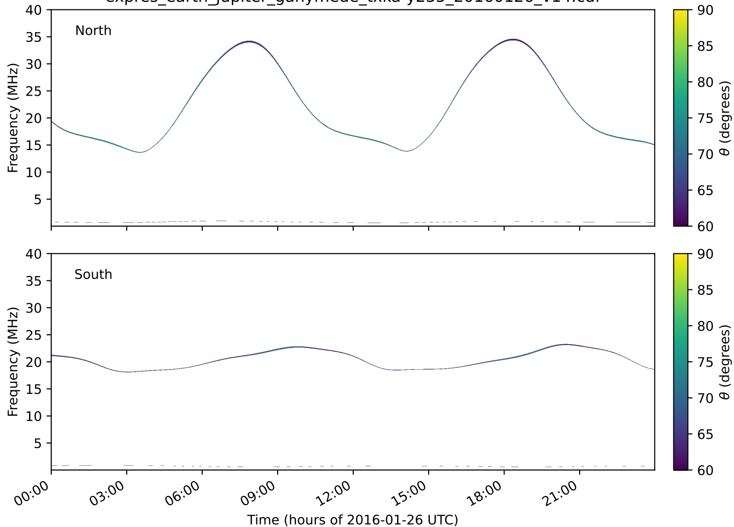
expres_earth_jupiter_ganymede_txka-y235_20160126_v14.cdf
