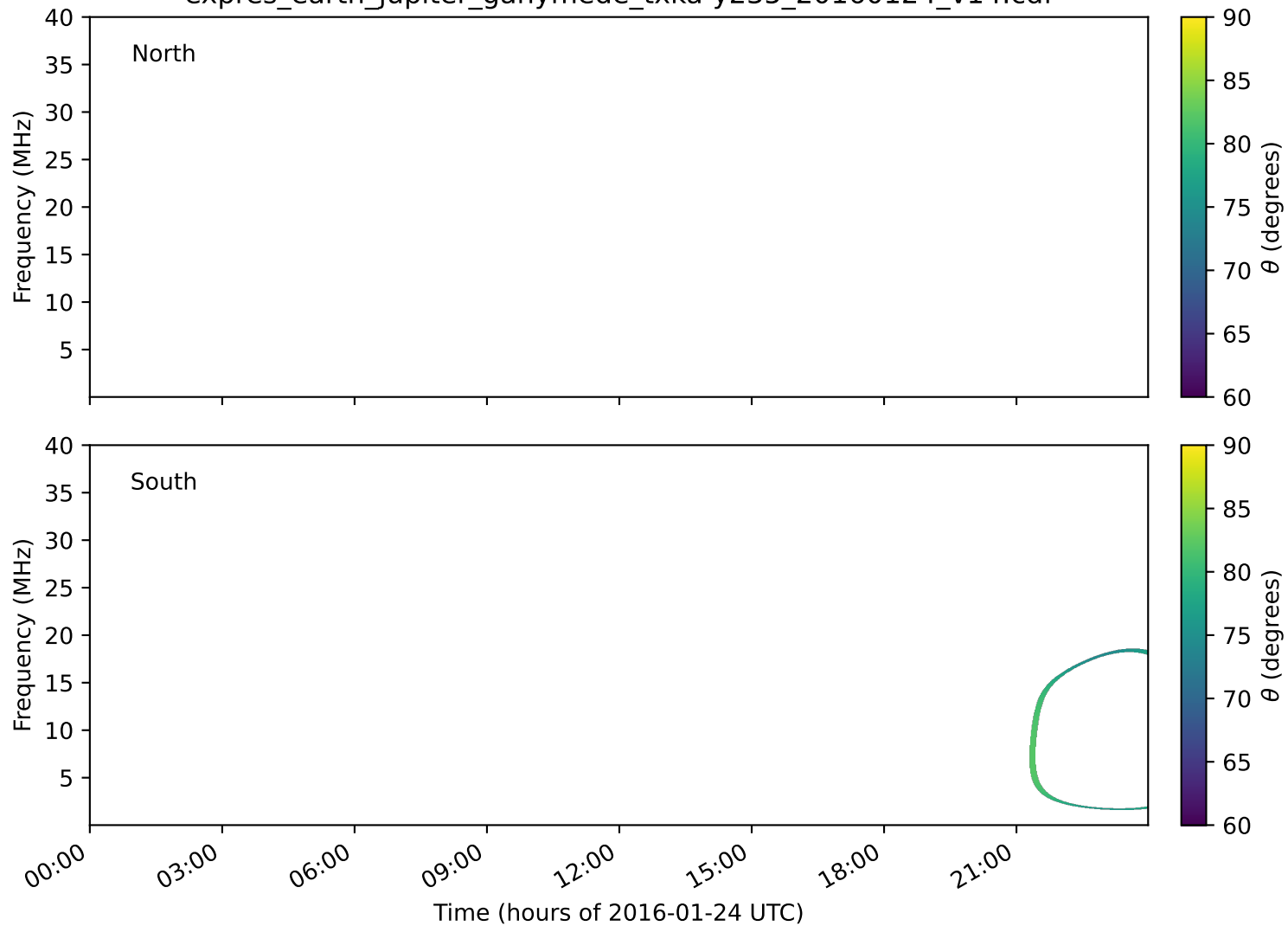
expres_earth_jupiter_ganymede_txka-y235_20160124_v14.cdf
