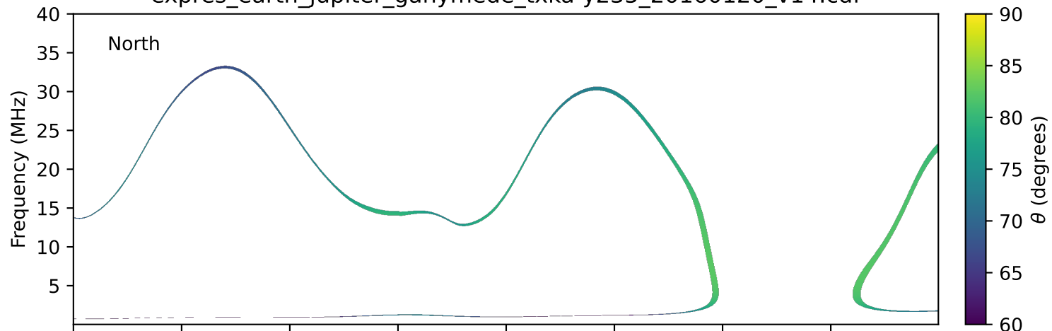
expres_earth_jupiter_ganymede_txka-y235_20160120_v14.cdf
