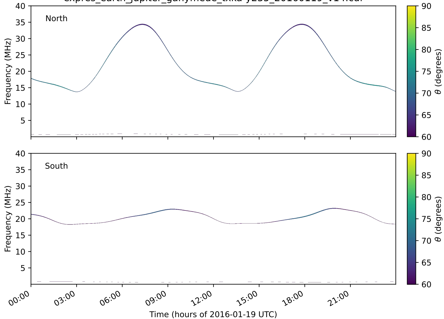
expres_earth_jupiter_ganymede_txka-y235_20160119_v14.cdf
