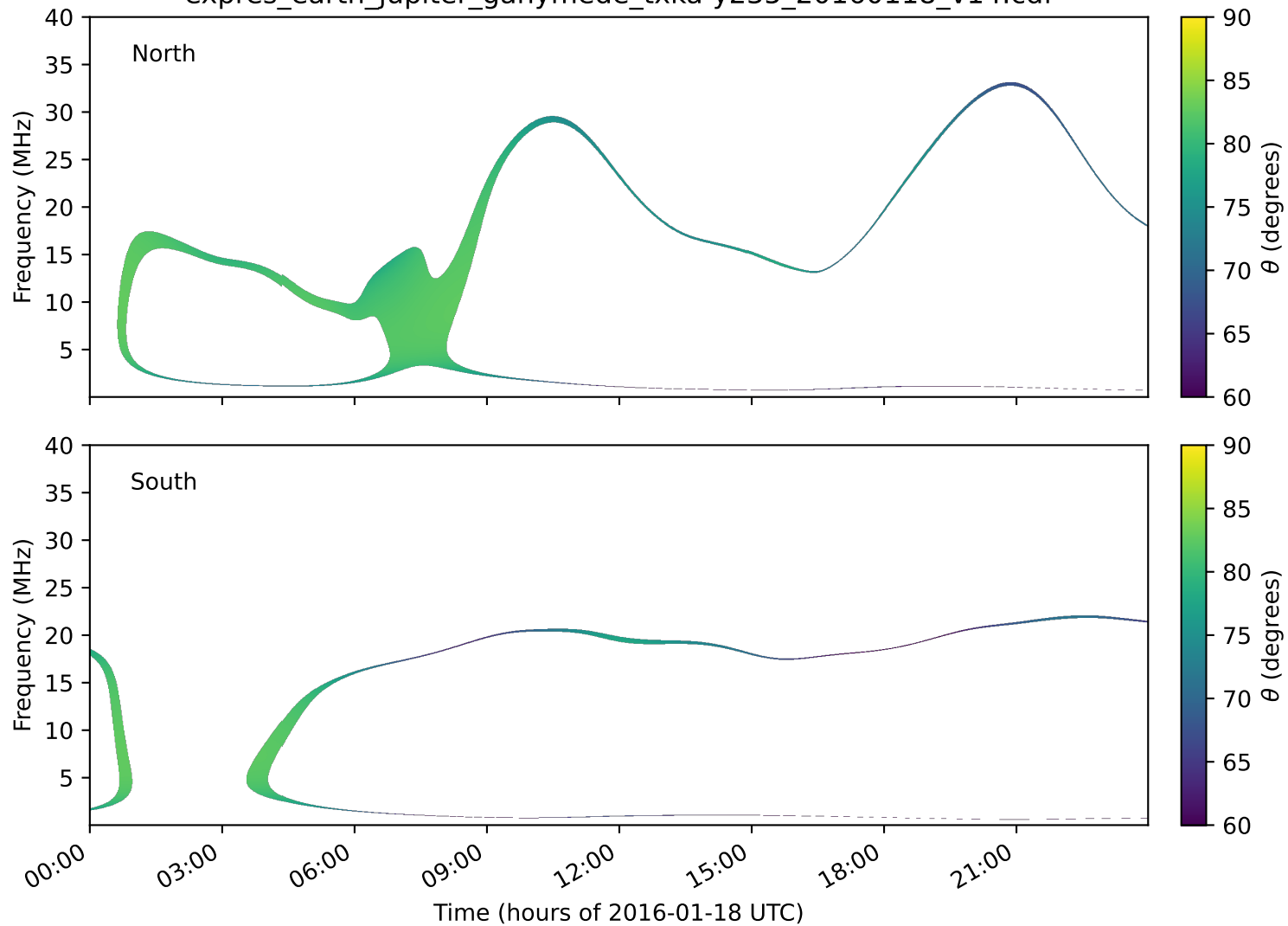
expres_earth_jupiter_ganymede_txka-y235_20160118_v14.cdf
