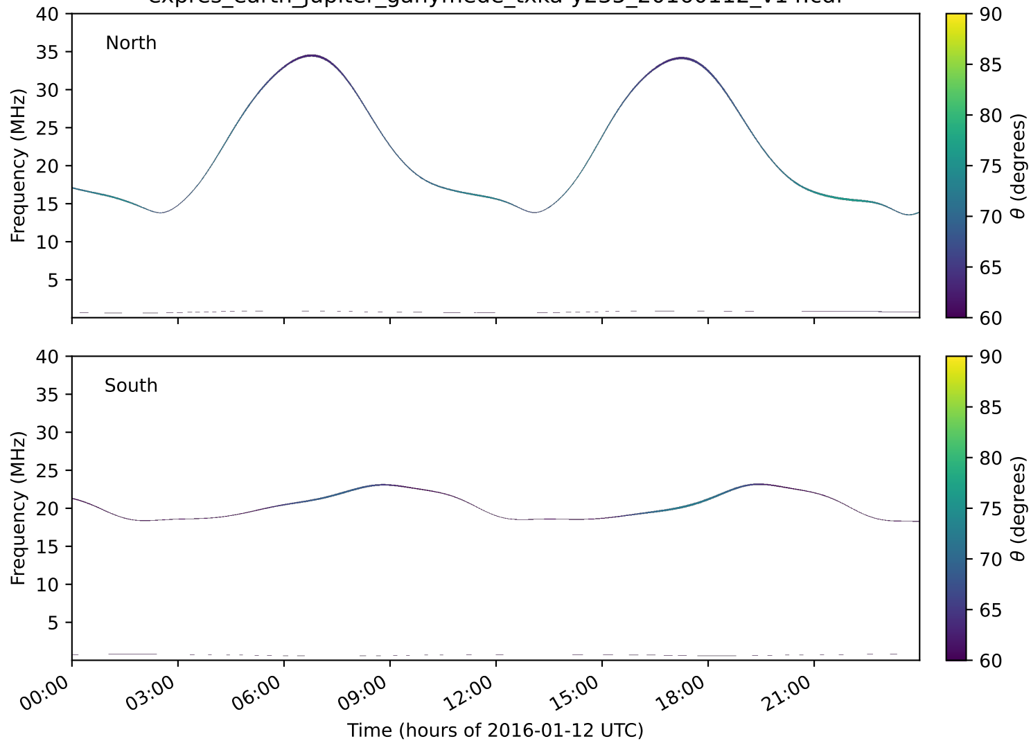
expres_earth_jupiter_ganymede_txka-y235_20160112_v14.cdf
