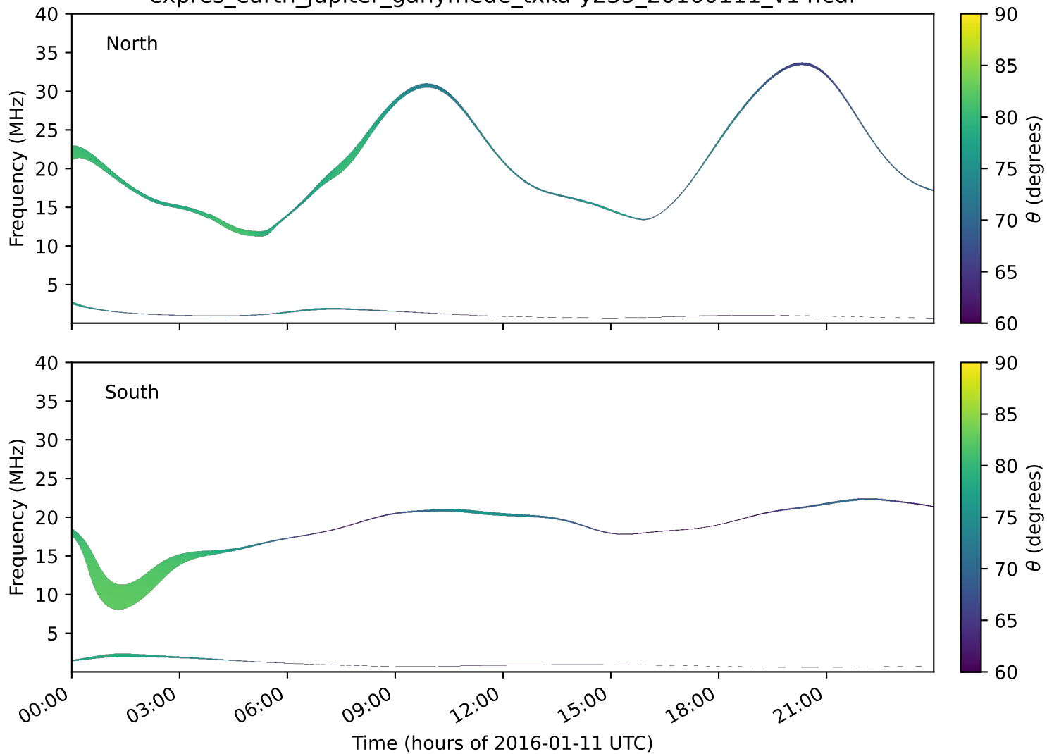
expres_earth_jupiter_ganymede_txka-y235_20160111_v14.cdf
