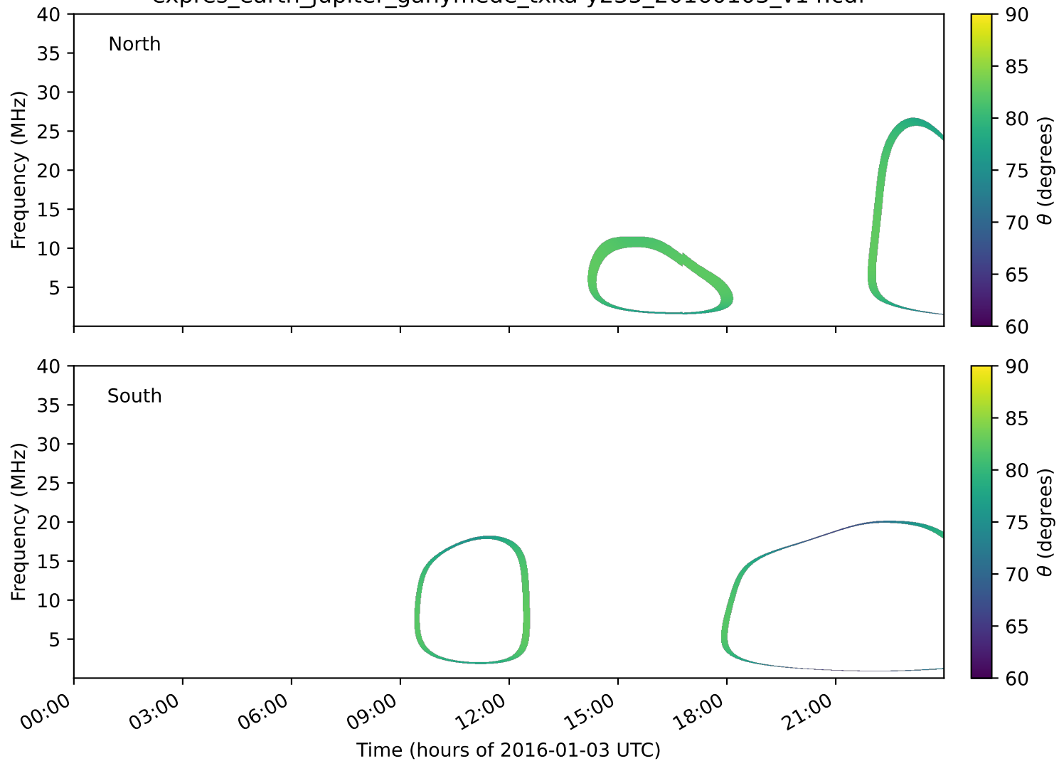
expres_earth_jupiter_ganymede_txka-y235_20160103_v14.cdf
