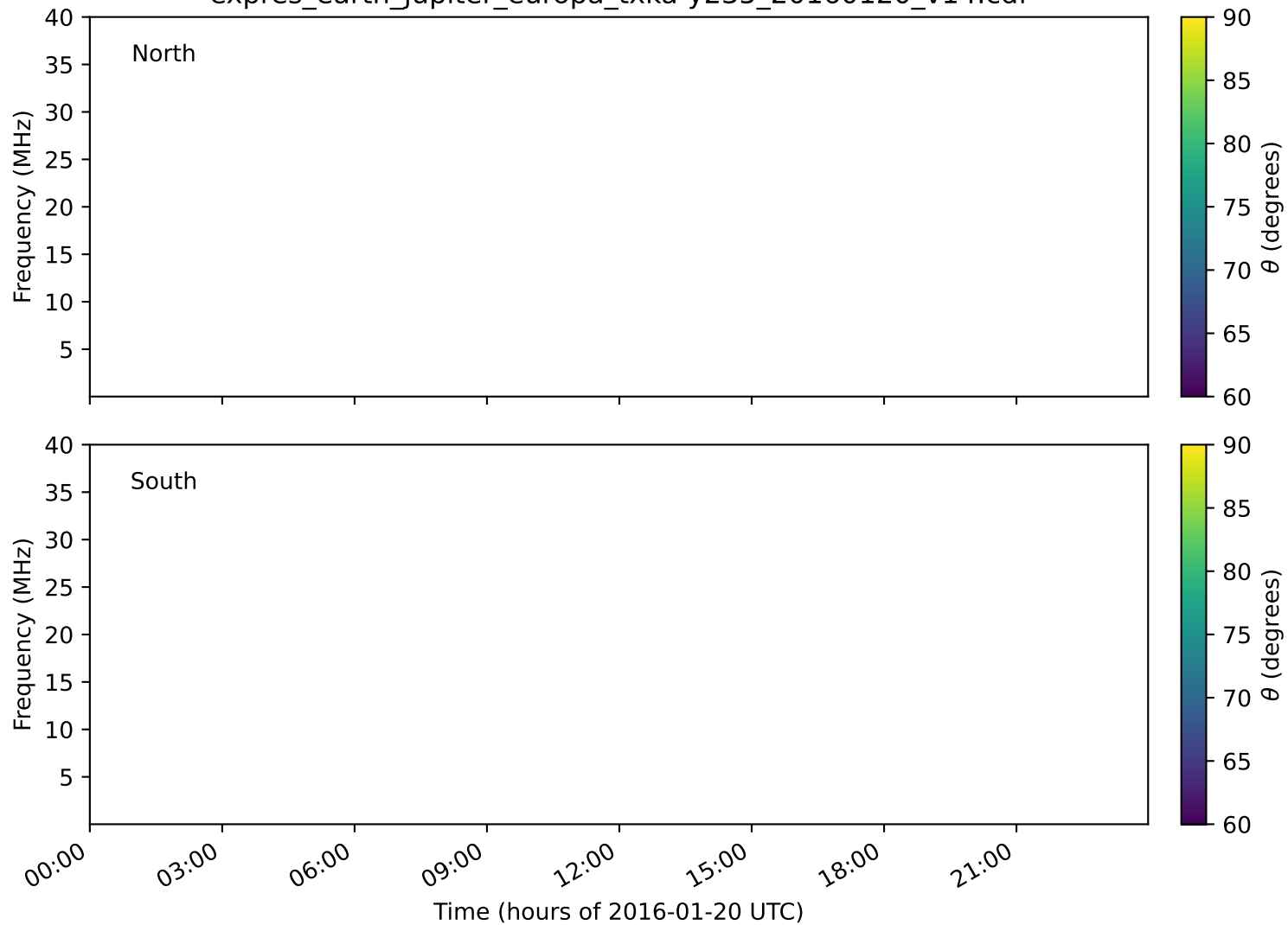
expres_earth_jupiter_europa_txka-y235_20160120_v14.cdf
