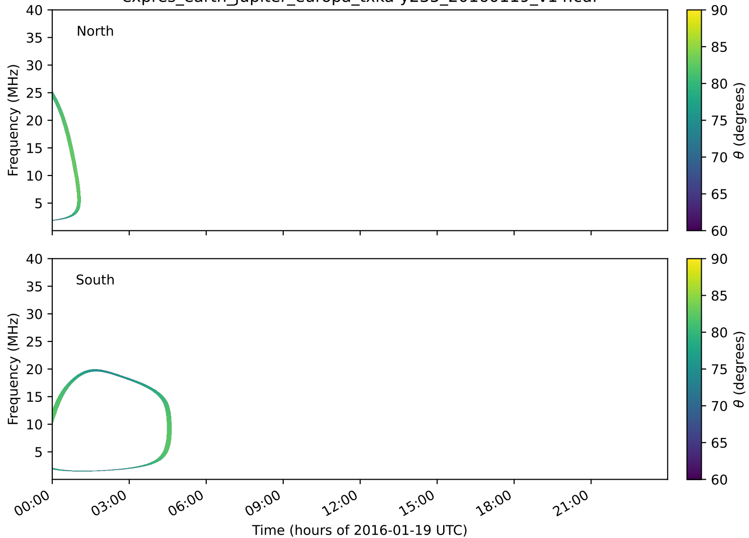
expres_earth_jupiter_europa_txka-y235_20160119_v14.cdf
