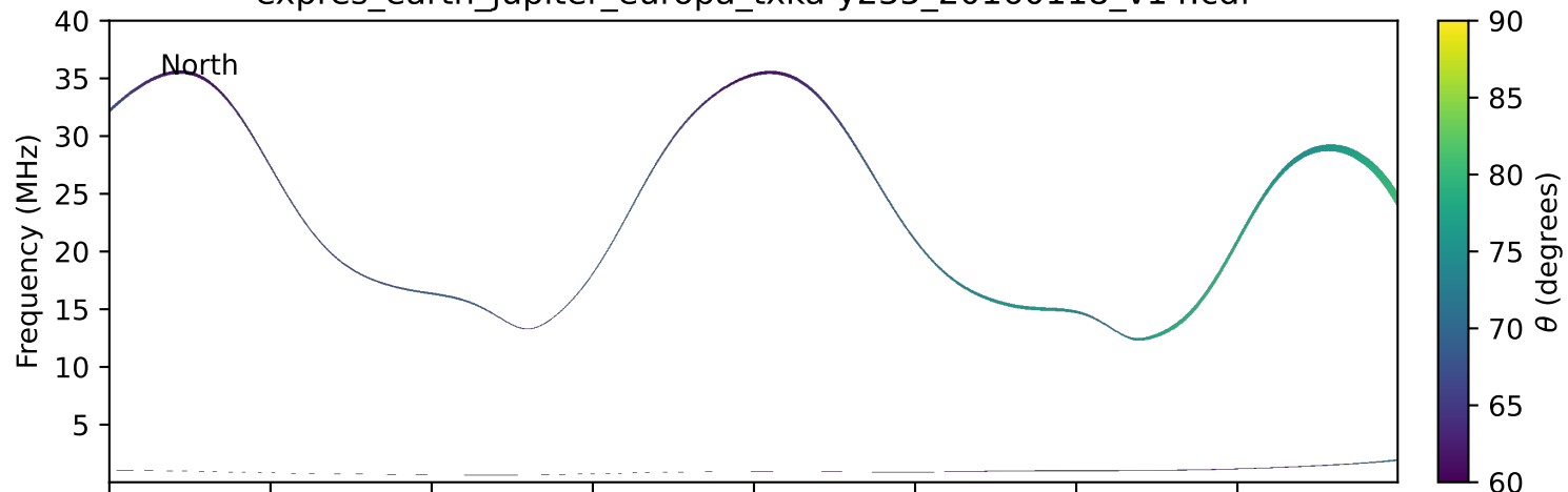
expres_earth_jupiter_europa_txka-y235_20160118_v14.cdf
