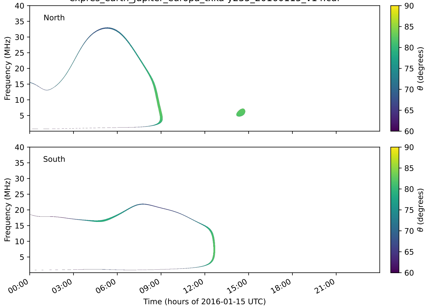
expres_earth_jupiter_europa_txka-y235_20160115_v14.cdf
