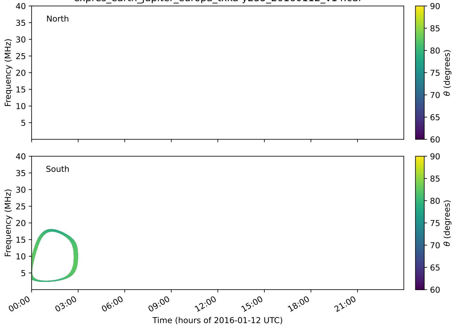
expres_earth_jupiter_europa_txka-y235_20160112_v14.cdf
