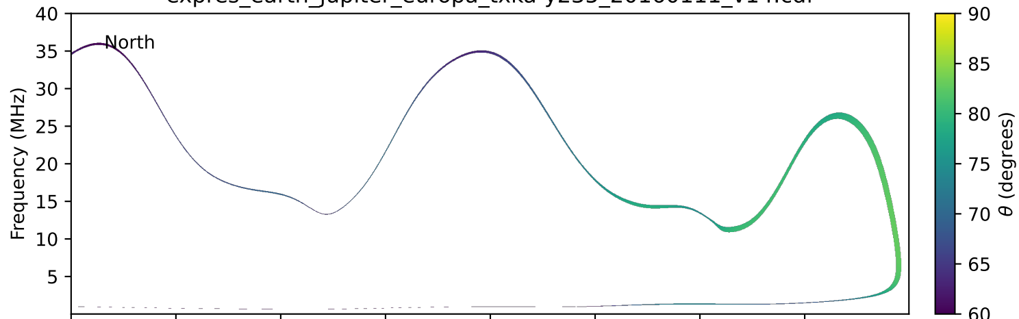
expres_earth_jupiter_europa_txka-y235_20160111_v14.cdf
