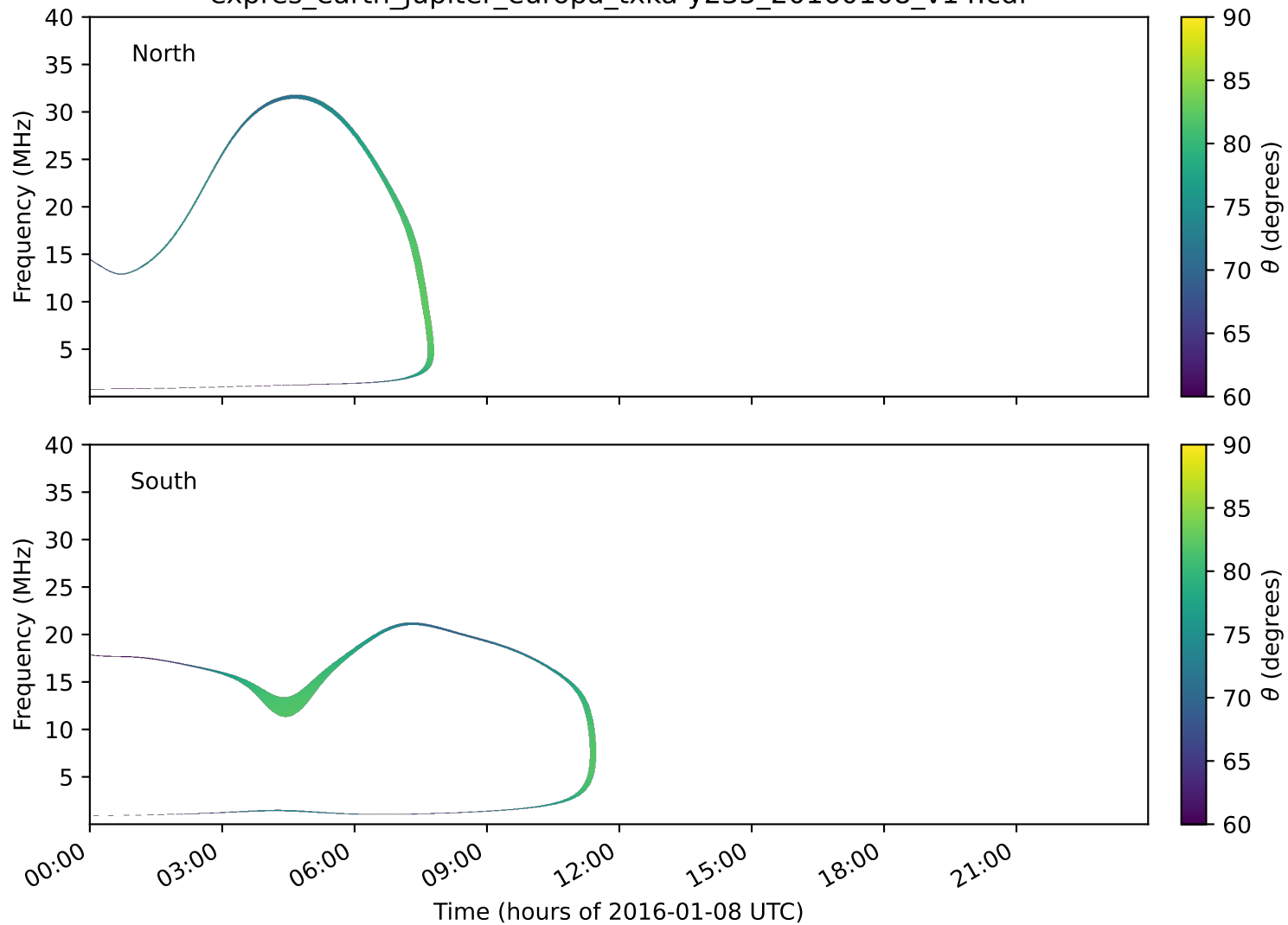
expres_earth_jupiter_europa_txka-y235_20160108_v14.cdf
