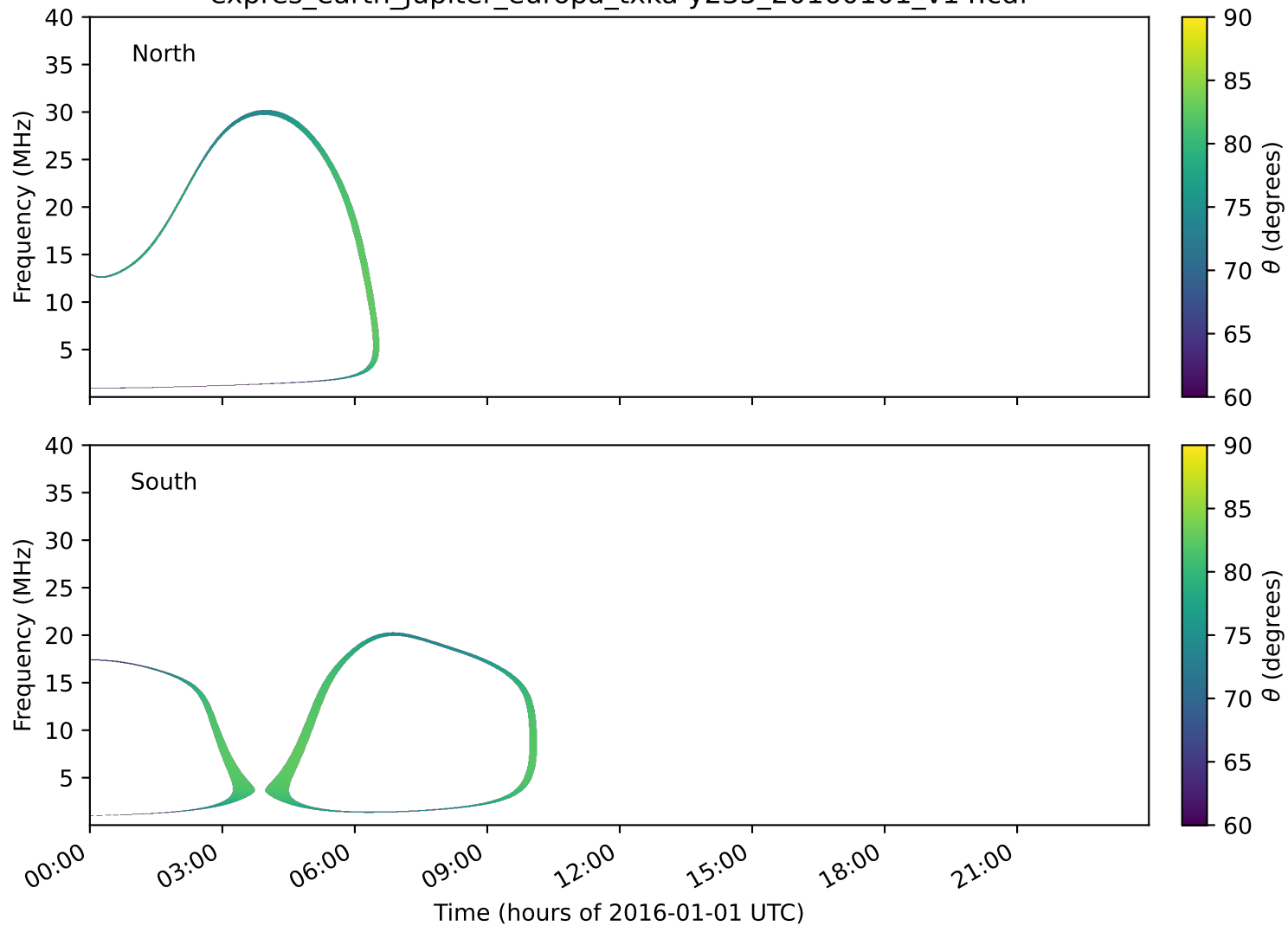
expres_earth_jupiter_europa_txka-y235_20160101_v14.cdf
