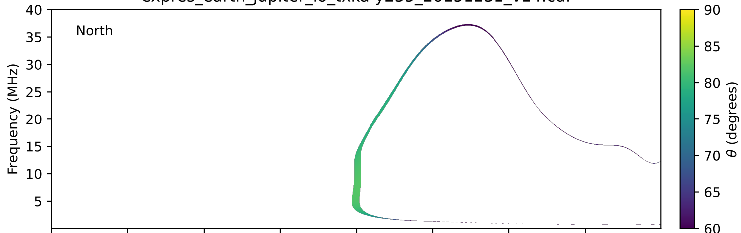
expres_earth_jupiter_io_txka-y235_20151231_v14.cdf
