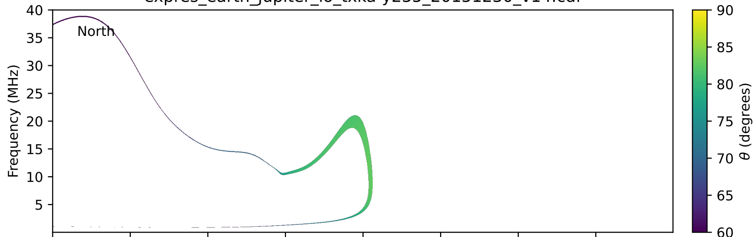
expres_earth_jupiter_io_txka-y235_20151230_v14.cdf
