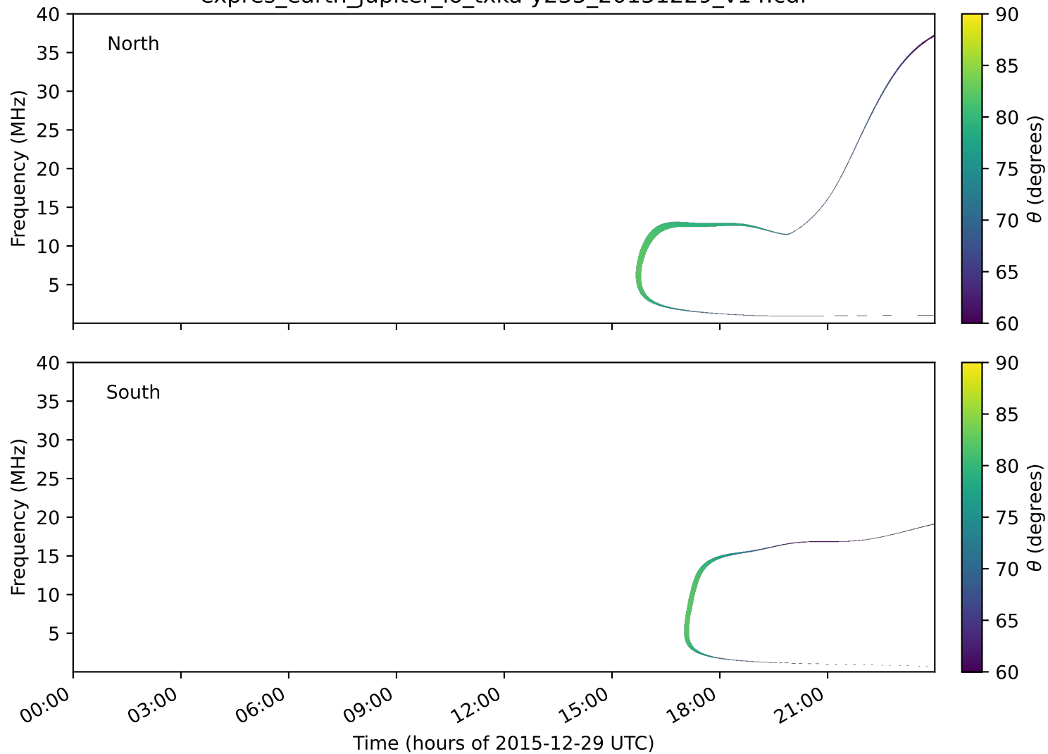
expres_earth_jupiter_io_txka-y235_20151229_v14.cdf
