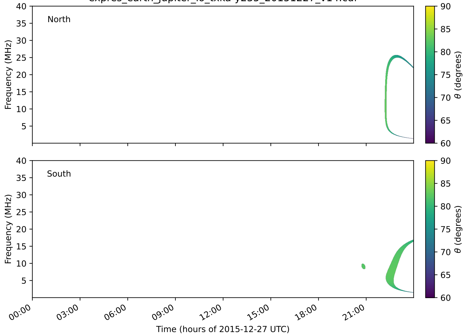
expres_earth_jupiter_io_txka-y235_20151227_v14.cdf
