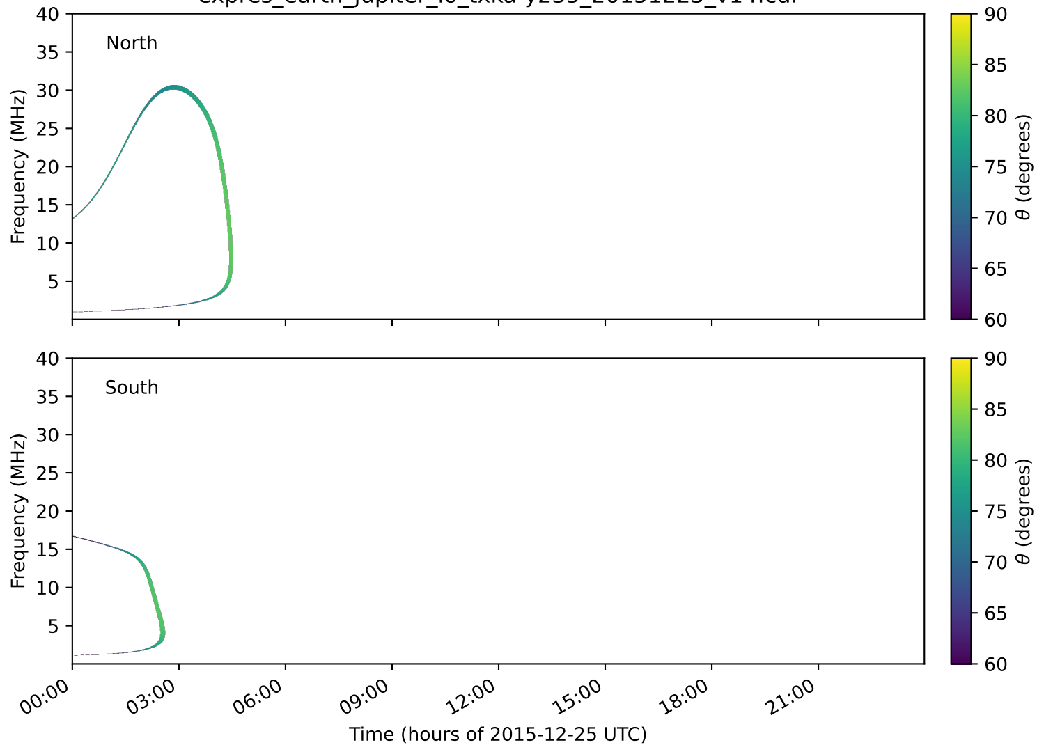
expres_earth_jupiter_io_txka-y235_20151225_v14.cdf
