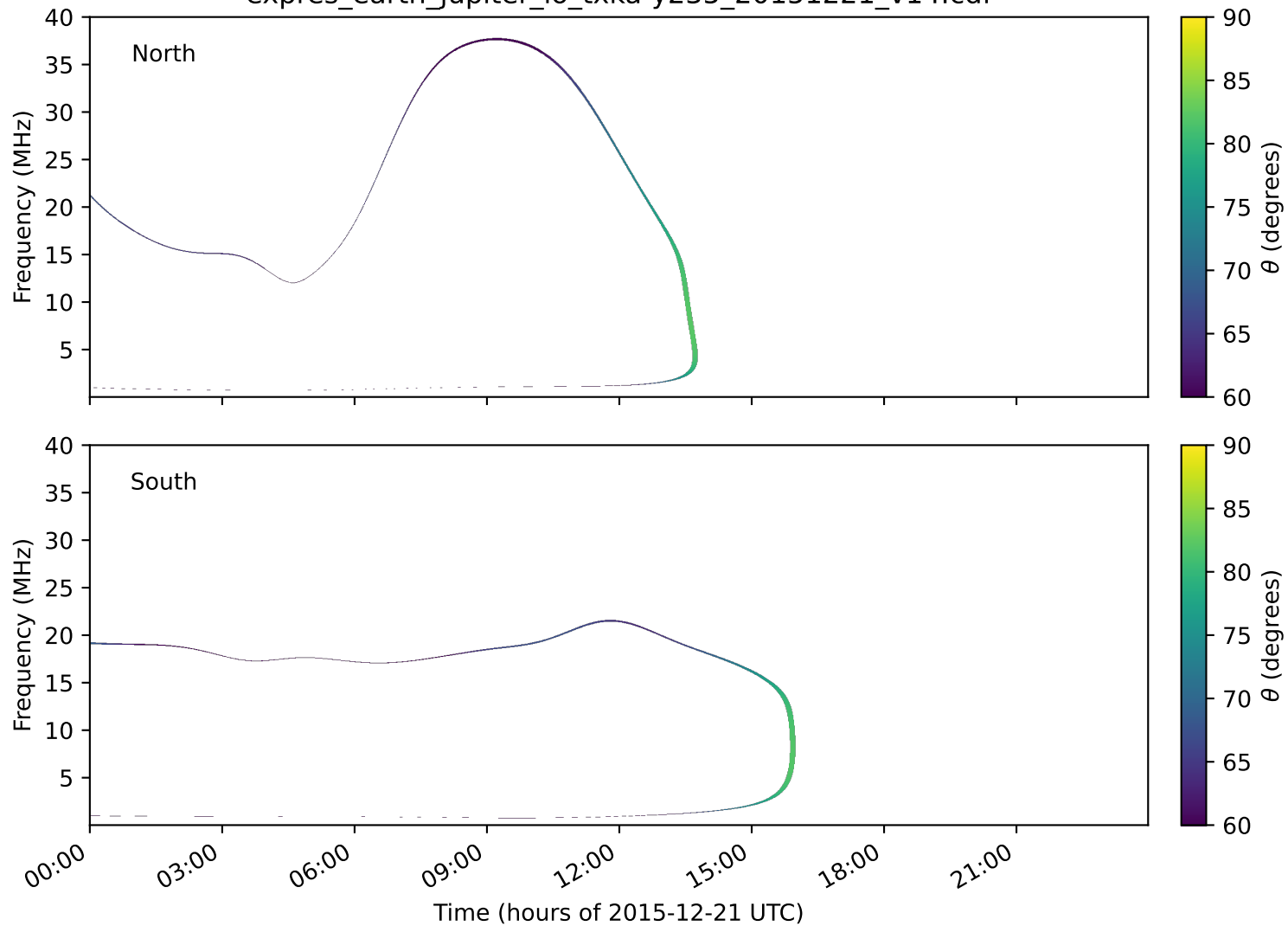
expres_earth_jupiter_io_txka-y235_20151221_v14.cdf
