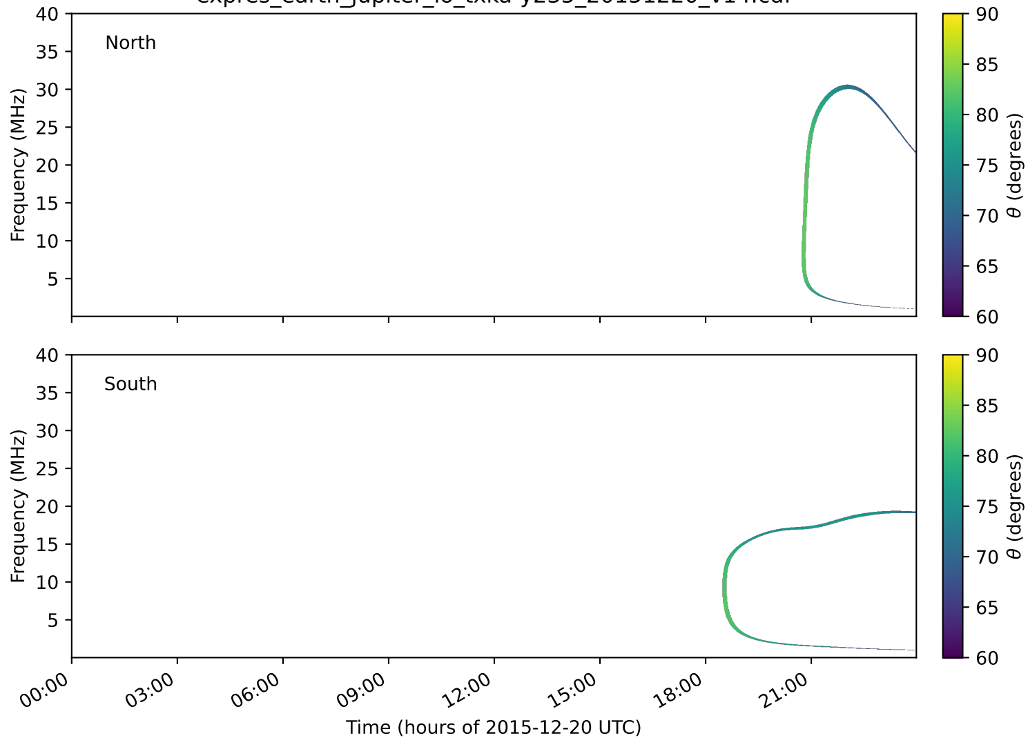
expres_earth_jupiter_io_txka-y235_20151220_v14.cdf
