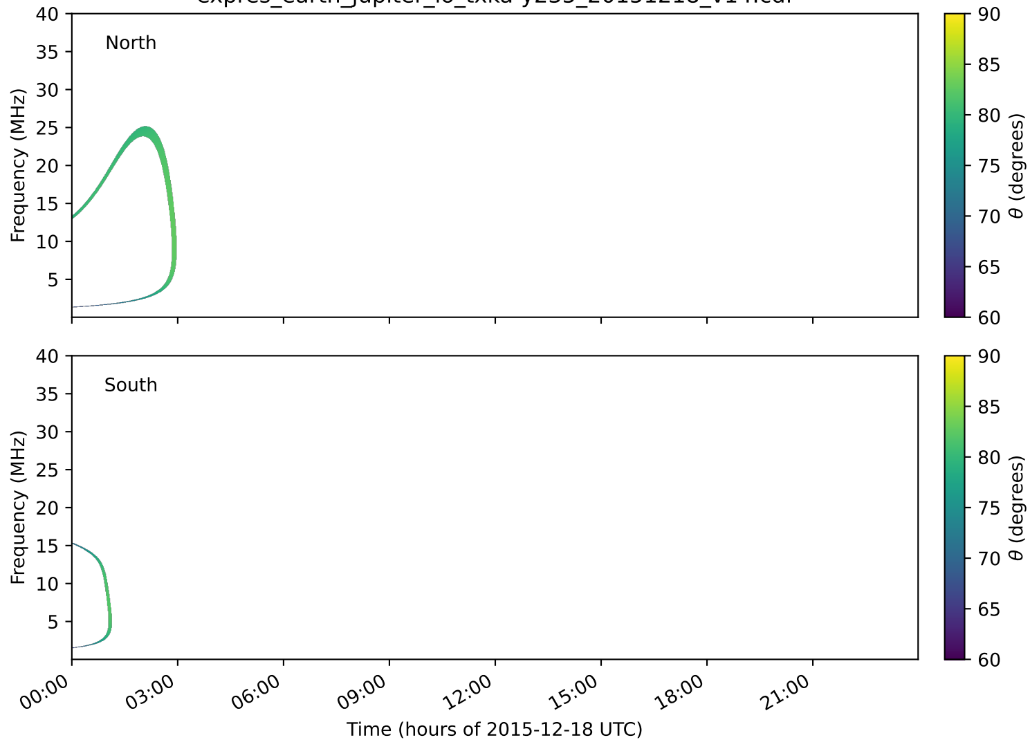
expres_earth_jupiter_io_txka-y235_20151218_v14.cdf
