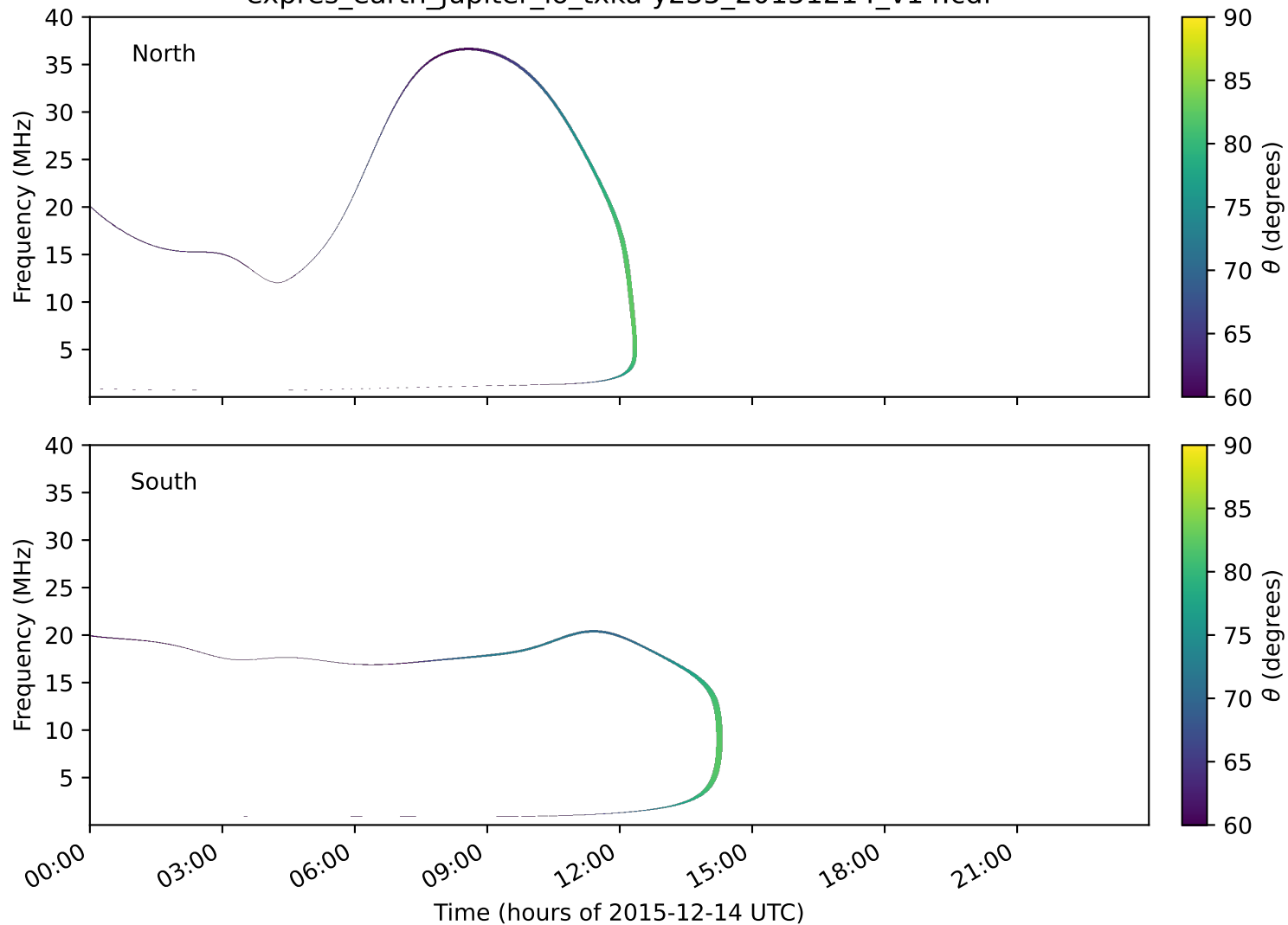
expres_earth_jupiter_io_txka-y235_20151214_v14.cdf
