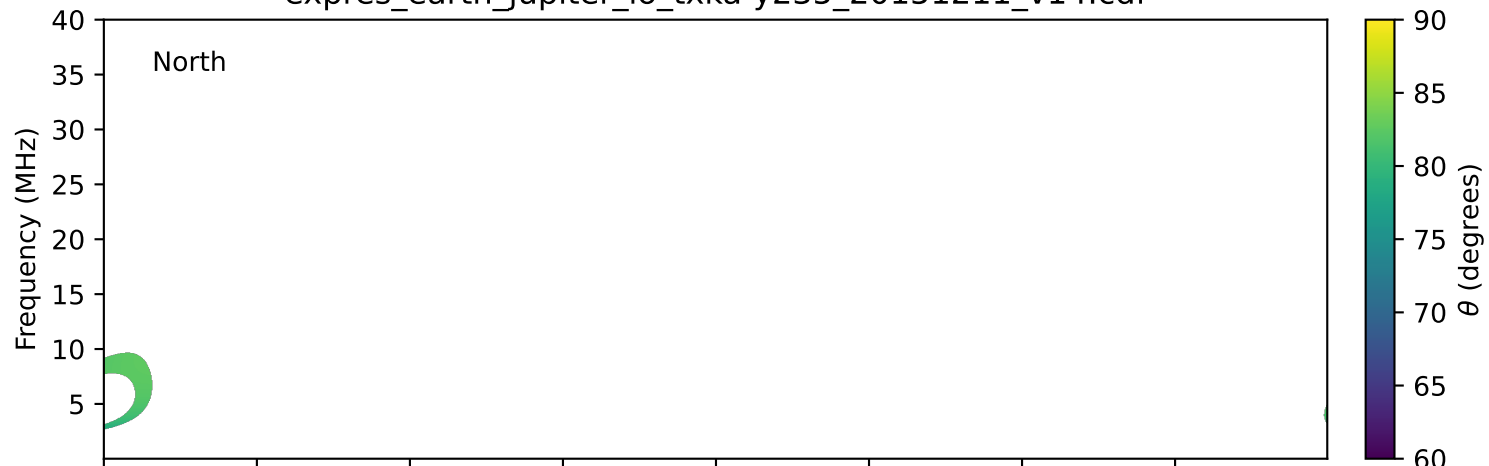
expres_earth_jupiter_io_txka-y235_20151211_v14.cdf
