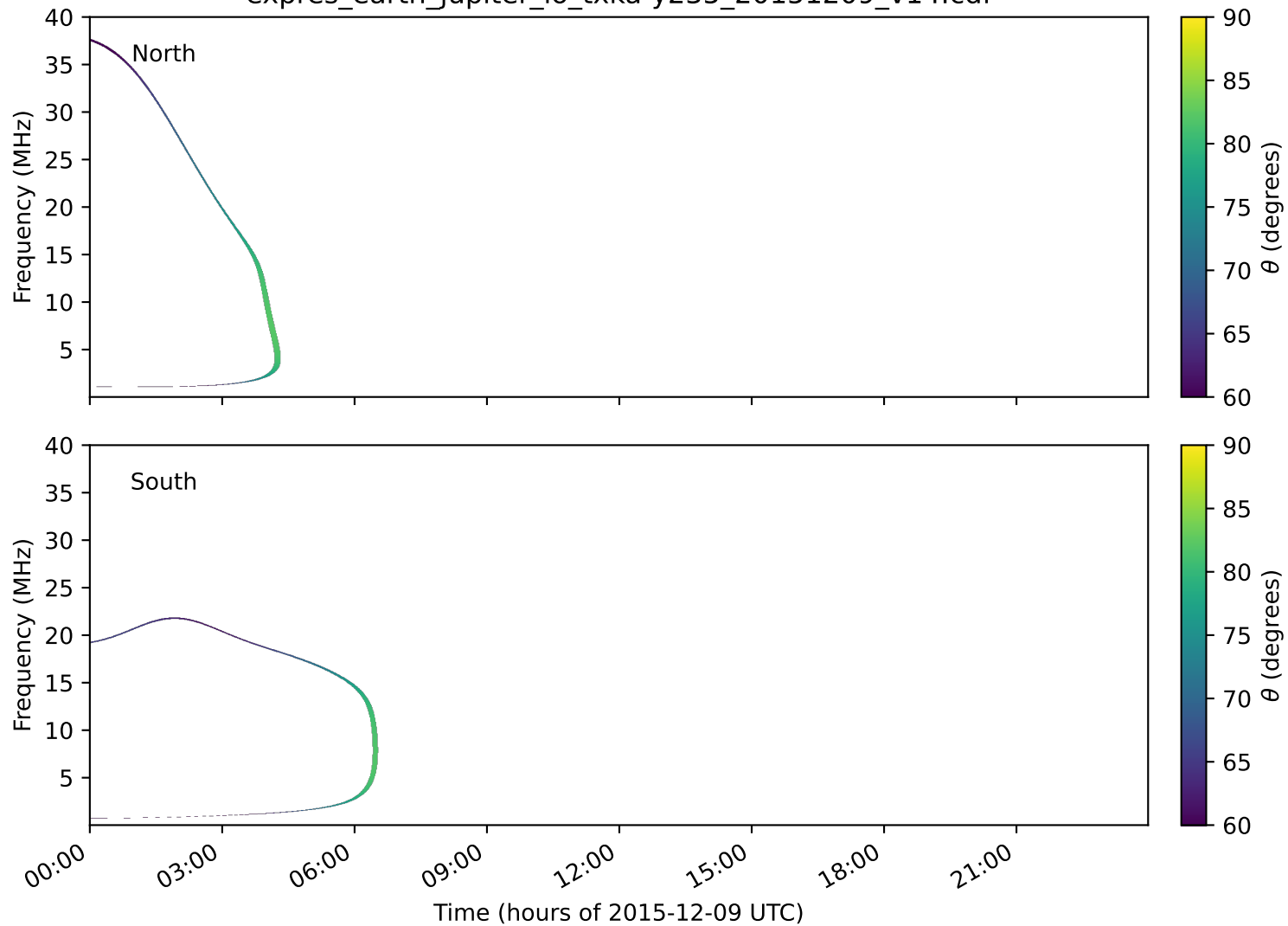
expres_earth_jupiter_io_txka-y235_20151209_v14.cdf
