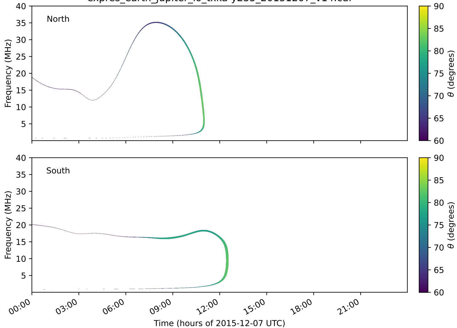
expres_earth_jupiter_io_txka-y235_20151207_v14.cdf
