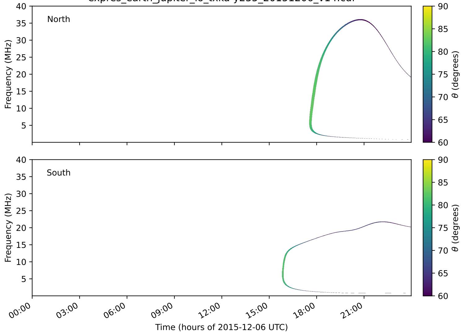
expres_earth_jupiter_io_txka-y235_20151206_v14.cdf
