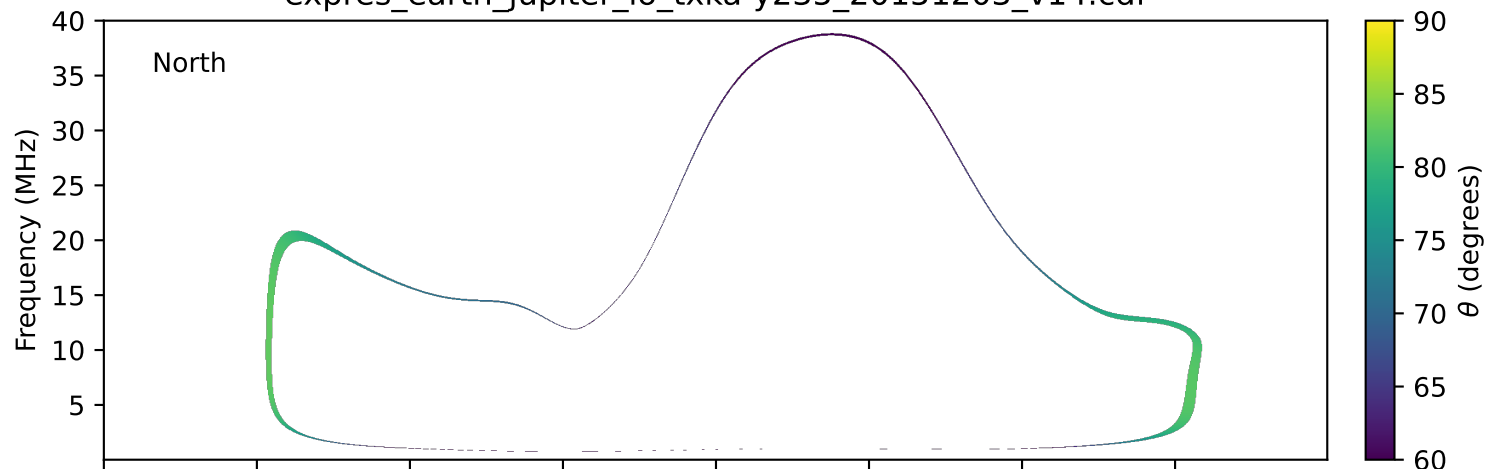
expres_earth_jupiter_io_txka-y235_20151203_v14.cdf
