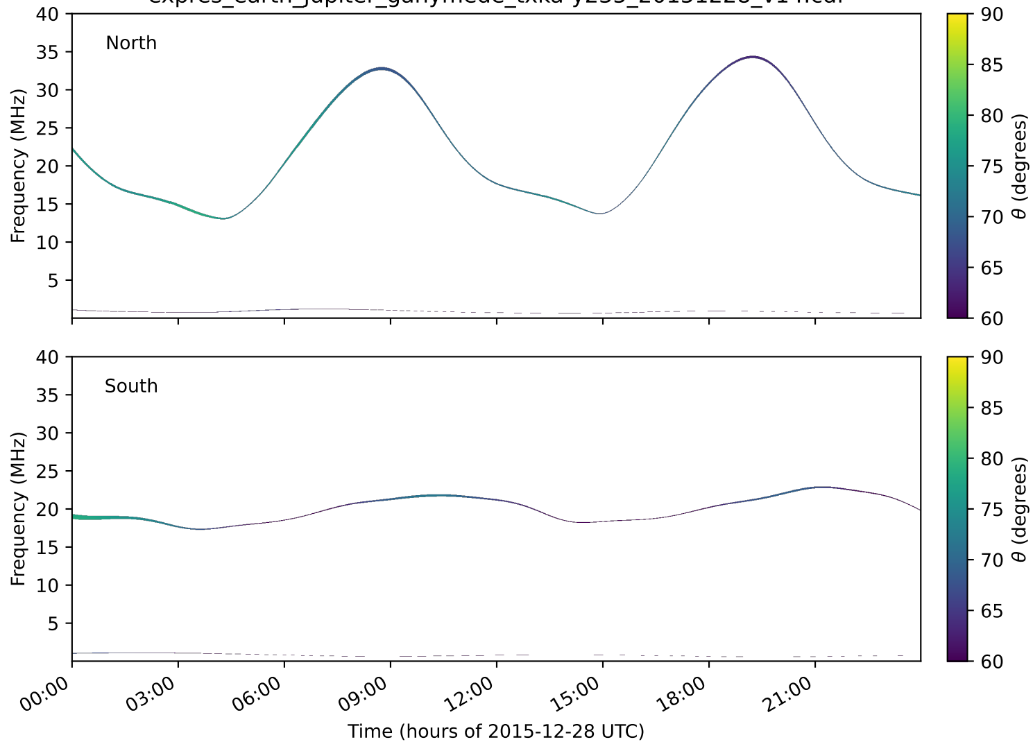
expres_earth_jupiter_ganymede_txka-y235_20151228_v14.cdf
