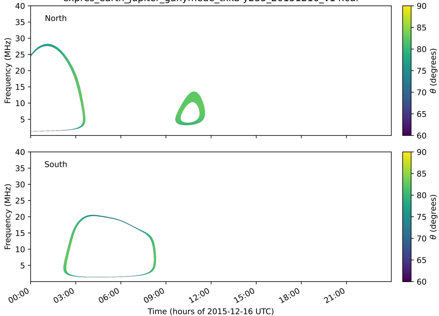
expres_earth_jupiter_ganymede_txka-y235_20151216_v14.cdf
