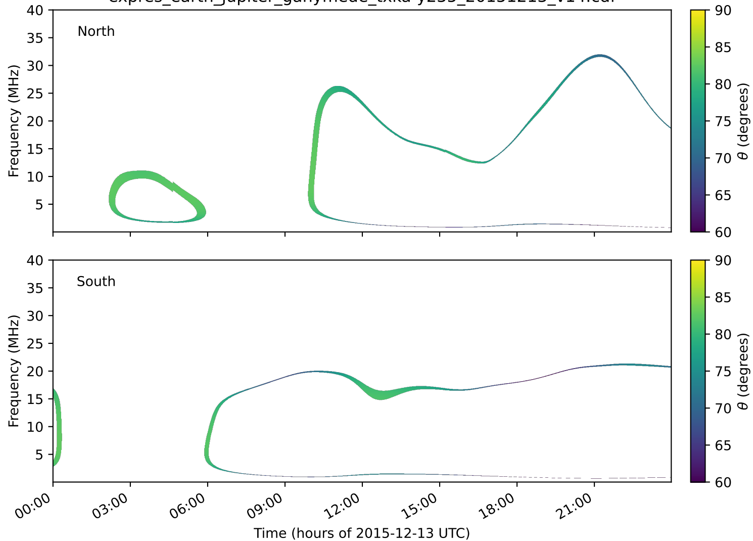
expres_earth_jupiter_ganymede_txka-y235_20151213_v14.cdf
