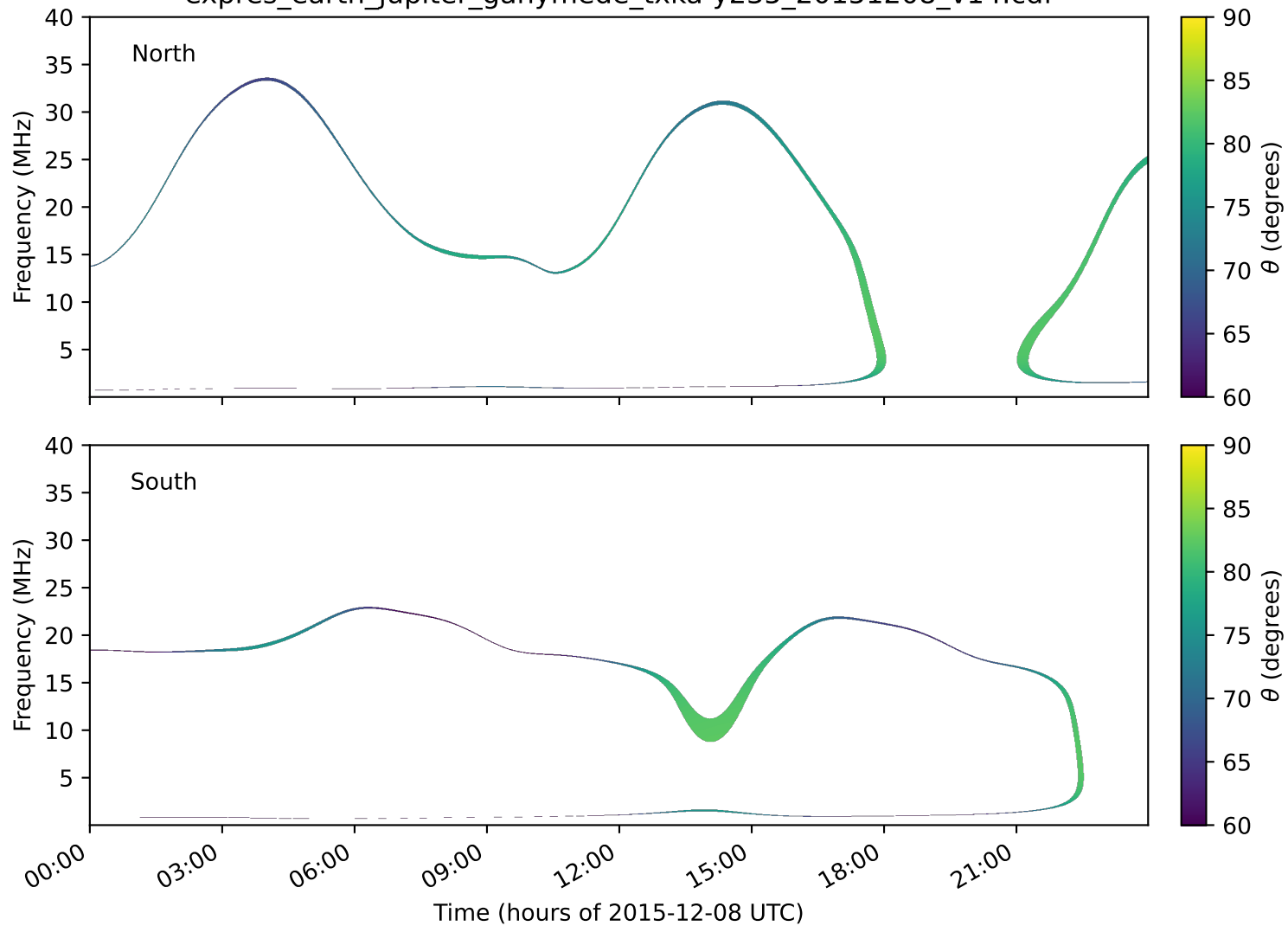
expres_earth_jupiter_ganymede_txka-y235_20151208_v14.cdf
