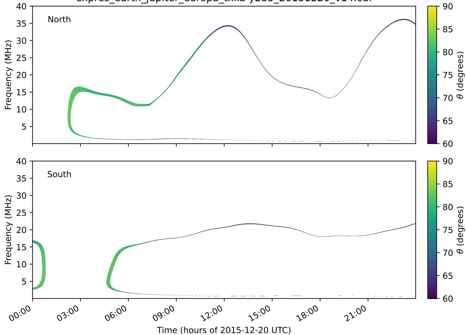
expres_earth_jupiter_europa_txka-y235_20151220_v14.cdf
