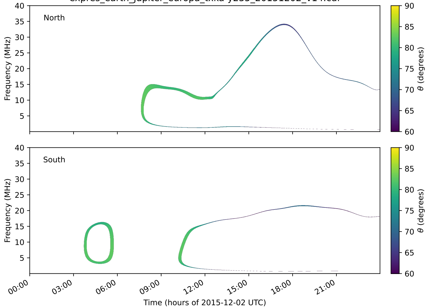
expres_earth_jupiter_europa_txka-y235_20151202_v14.cdf
