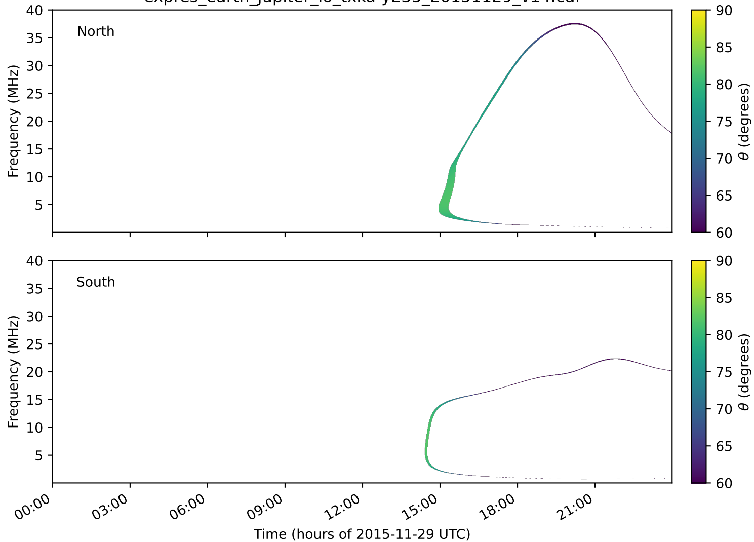
expres_earth_jupiter_io_txka-y235_20151129_v14.cdf
