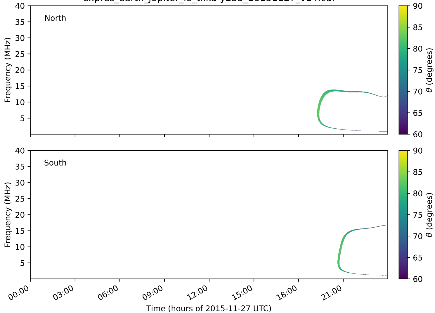
expres_earth_jupiter_io_txka-y235_20151127_v14.cdf
