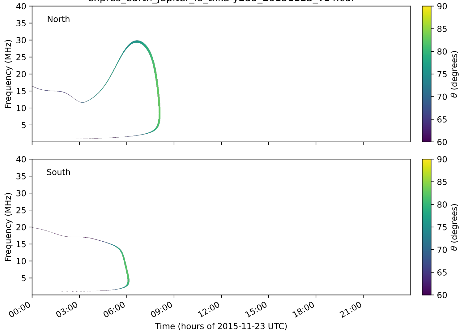
expres_earth_jupiter_io_txka-y235_20151123_v14.cdf
