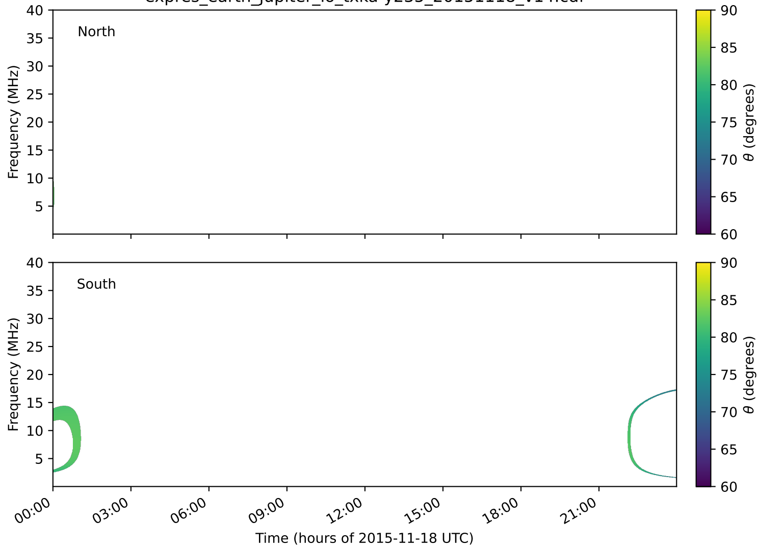
expres_earth_jupiter_io_txka-y235_20151118_v14.cdf
