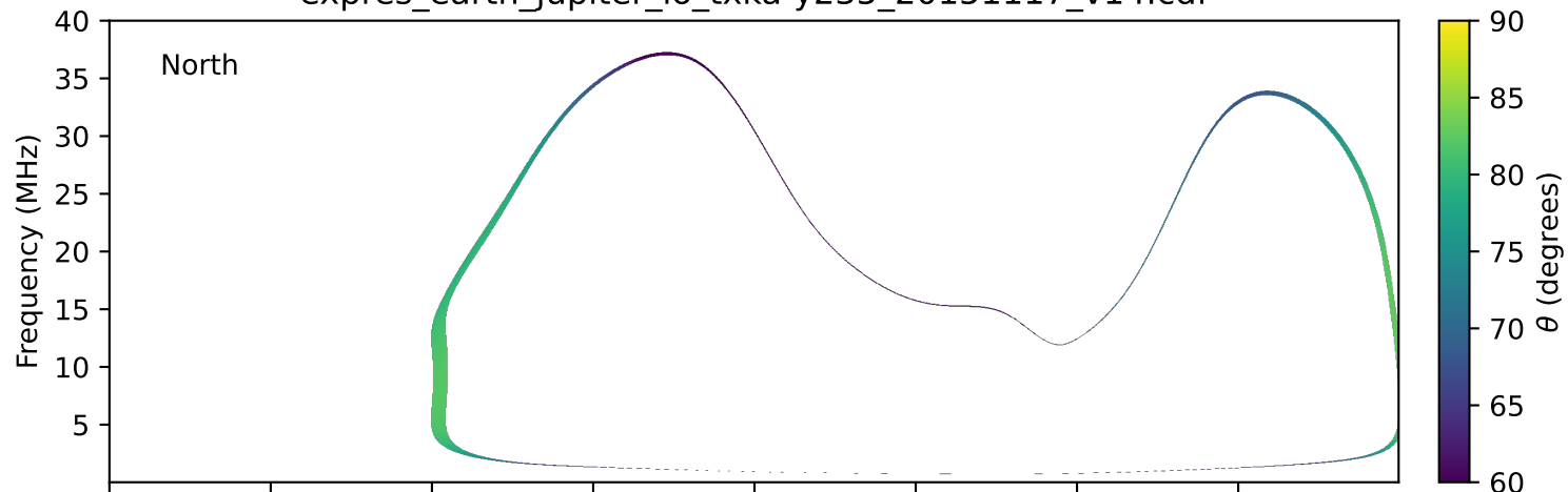
expres_earth_jupiter_io_txka-y235_20151117_v14.cdf
