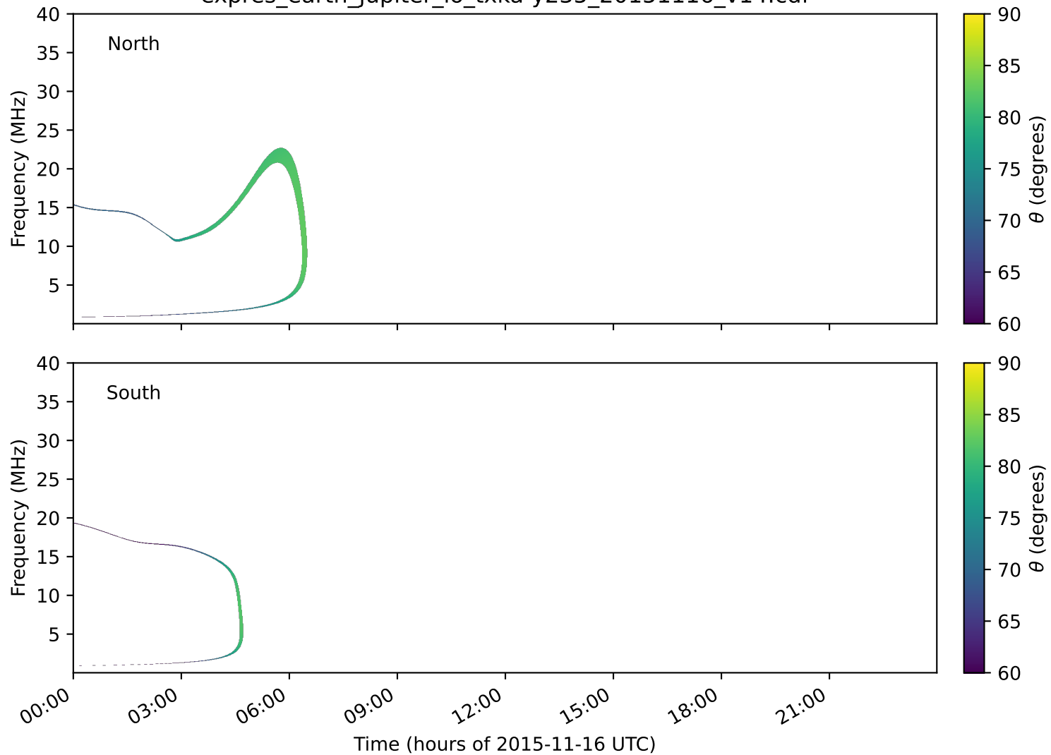
expres_earth_jupiter_io_txka-y235_20151116_v14.cdf
