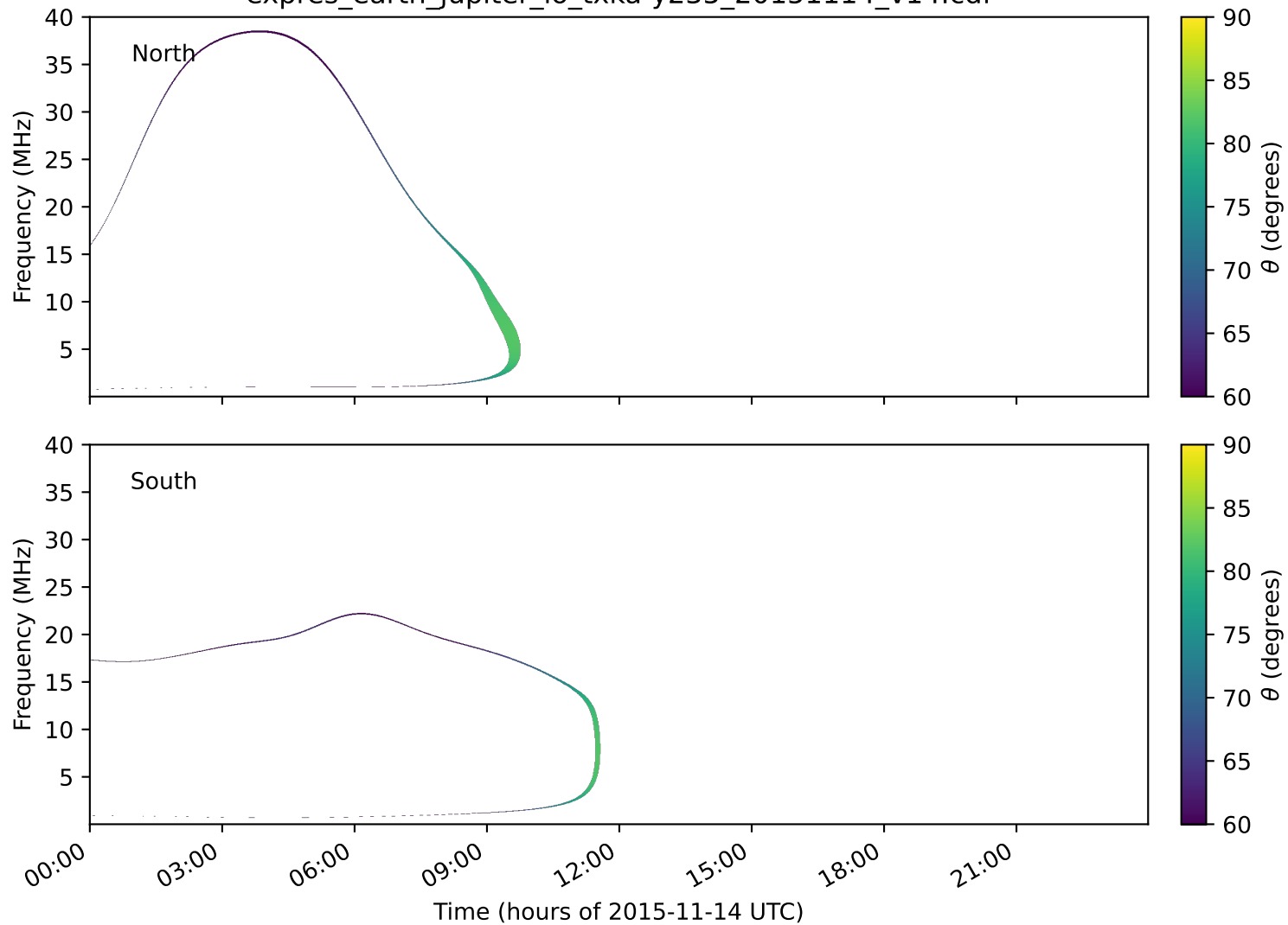
expres_earth_jupiter_io_txka-y235_20151114_v14.cdf
