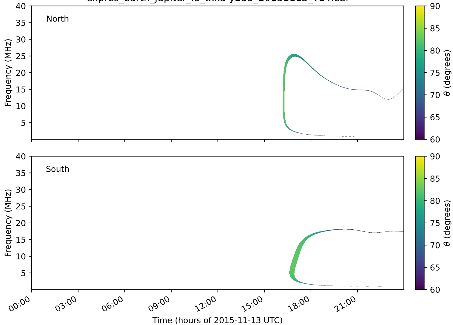
expres_earth_jupiter_io_txka-y235_20151113_v14.cdf
