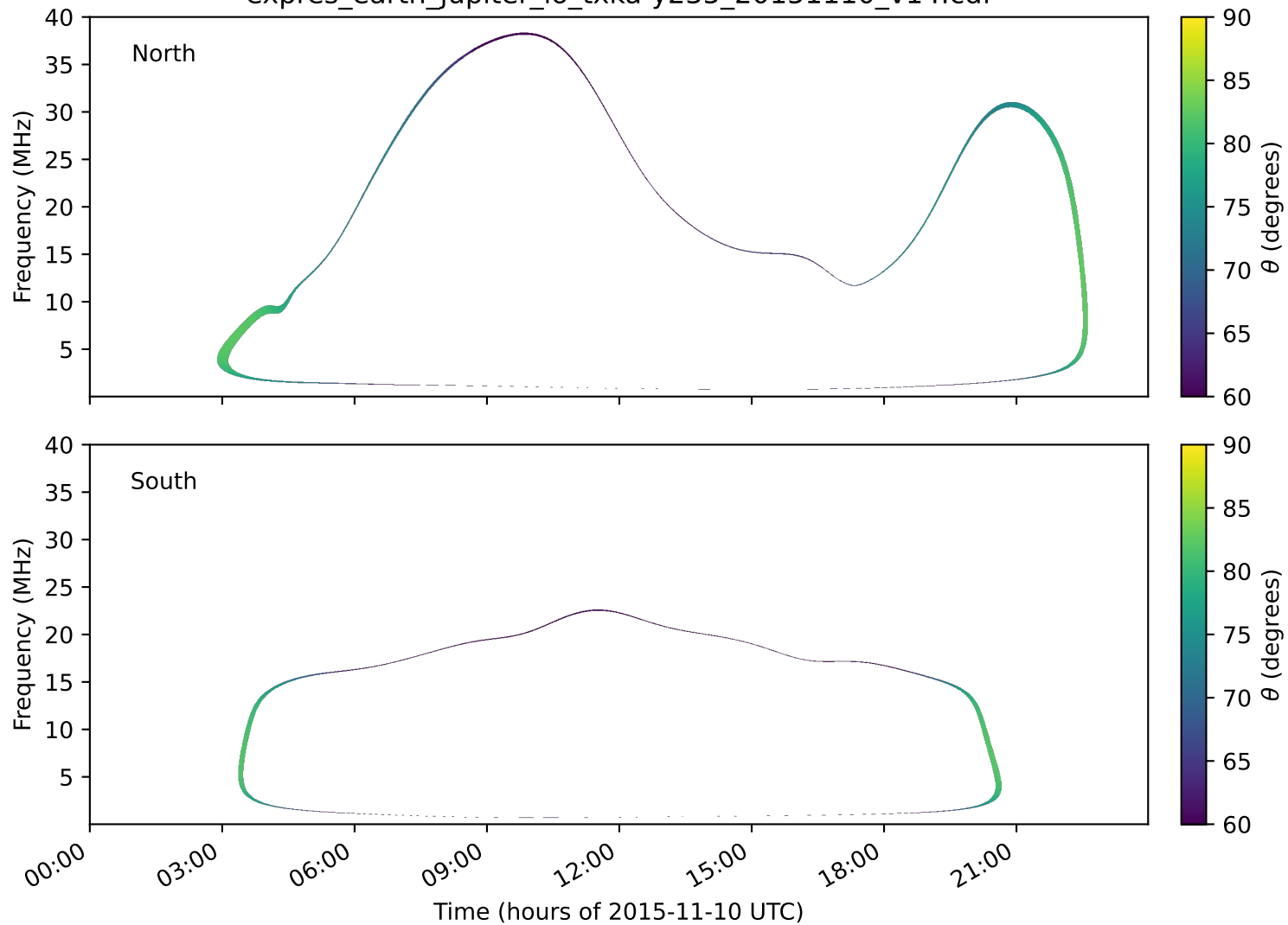
expres_earth_jupiter_io_txka-y235_20151110_v14.cdf
